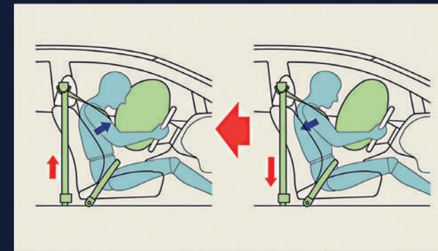
3-POINT ELR FRONT SEATBELTS WITH PRETENSIONER AND FORCE LIMITER 3-POINT ELR REAR SEATBELTS FRONT SEATBELT REMINDER
